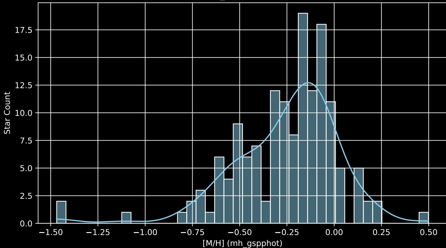
APOGEE DR17 Field: [047-26_MGA [M/H] (mh_gspphot) (n= 150)
