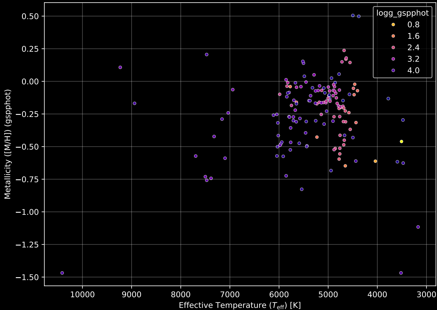
APOGEE DR17 Field: [047-26_MGA] Stellar Population Parameters (n= 151)
