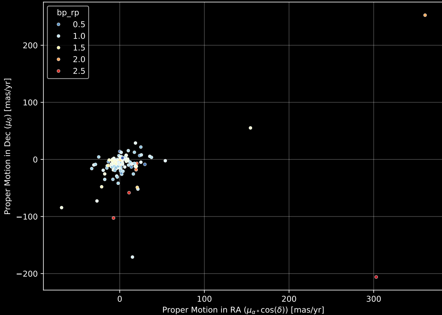
APOGEE DR17 Field: [047-26_MGA] Proper Motion Diagram (n= 151)
