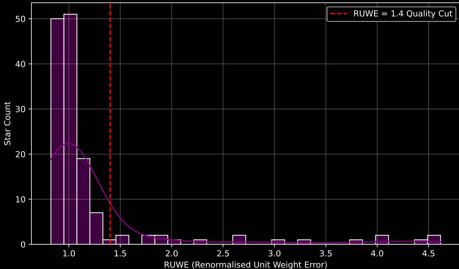
GAPOGEE DR17 Field [047-26_MGA] RUWE Distribution (n= 146)
