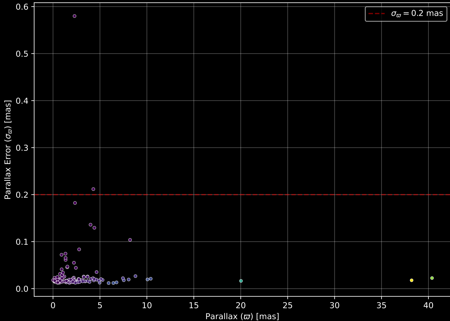
APOGEE DR17 Field: [047-26_MGA] Parallax Quality (n= 151)
