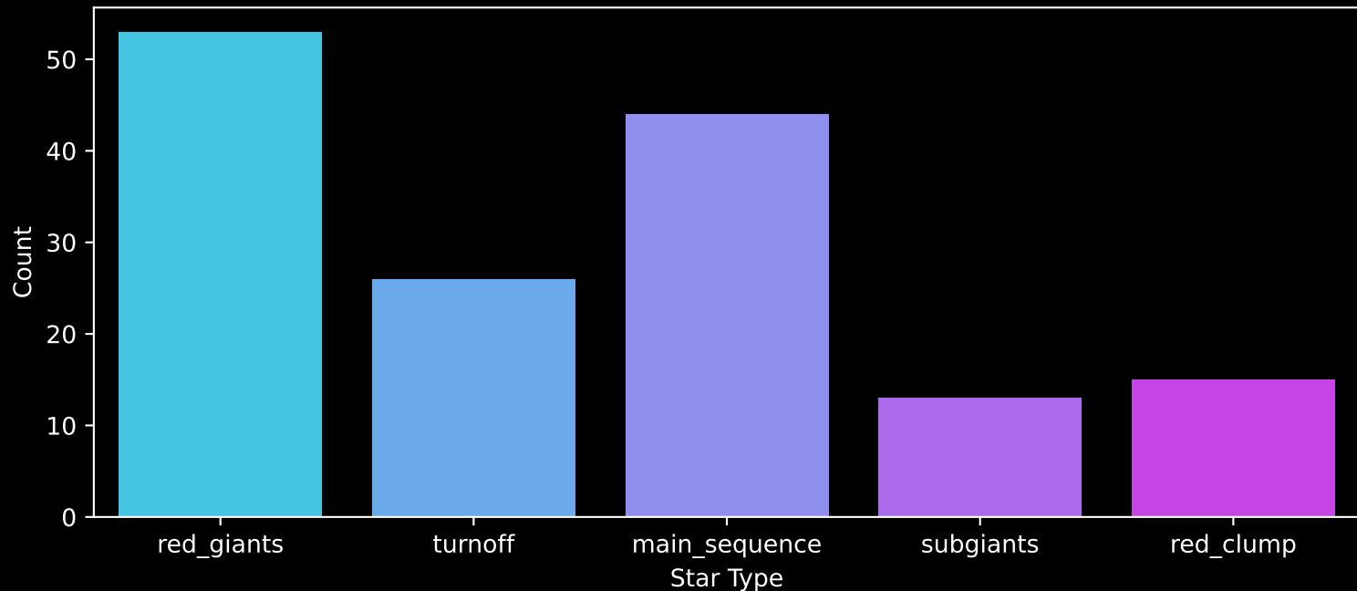
APOGEE DR17 Field: [047-26_MGA] Count plot of Star Type
